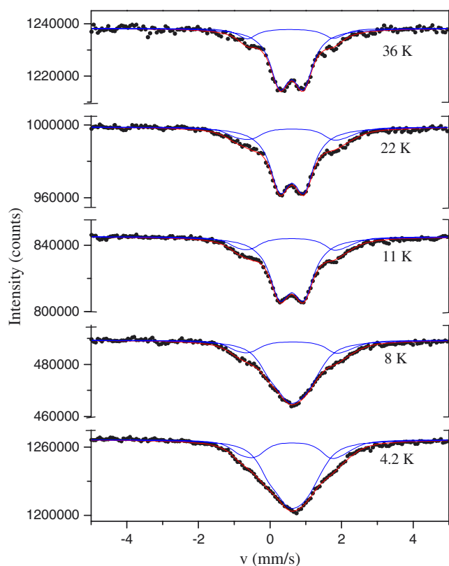
Figure 6. ^{155}\text{Gd} Mössbauer spectra of \text{GdCrO}_4 at different temperatures between 4.2 and 36 K. The ratio of the two subspectra turns out to be 80–20%.
