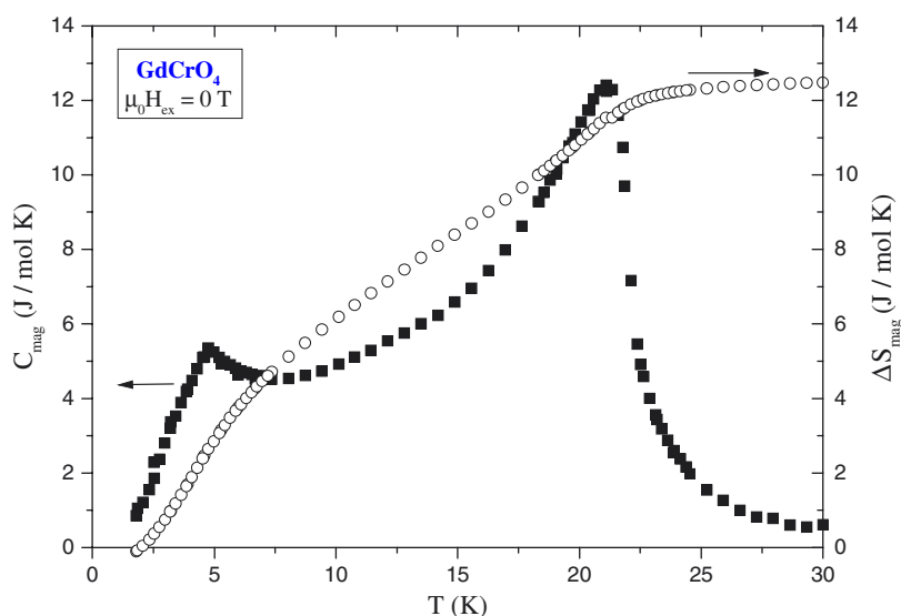
Figure 4. Magnetic contribution to the specific heat of GdCrO 4 between 2 and 30 K in the absence of an applied magnetic field, coupled with the associated variation of entropy.
