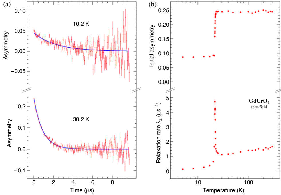
Figure 8. (a) \mu SR spectra of GdCrO 4 measured at T = 10.2 and 30.2 K. (b) Variation of both the initial asymmetry ( a_0 ) and the relaxation rate ( \lambda_z ) with temperature. The magnetic ordering temperature obtained from these \mu SR experiments is 22.6 K.
