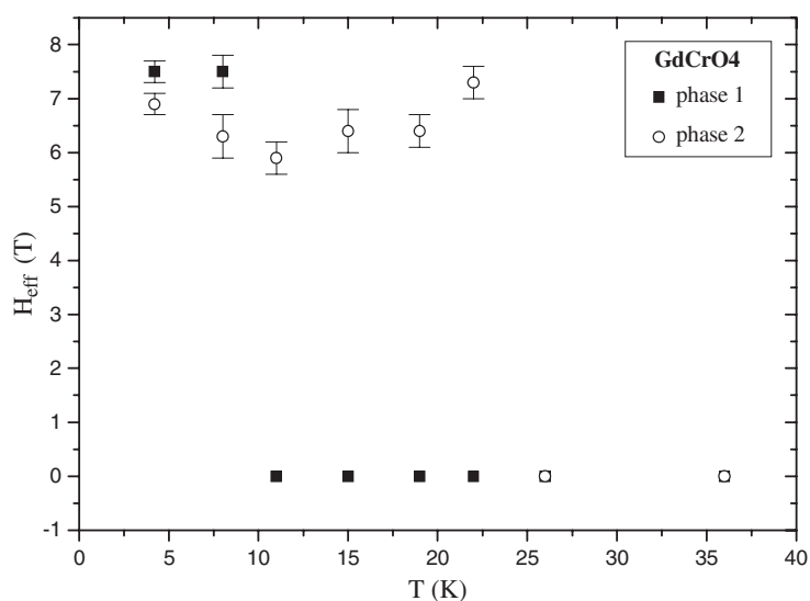
Figure 7. Temperature dependence of the hyperfine magnetic field of both the orthorhombic (1) and the tetragonal (2) phases present in GdCrO 4 between 4.2 and 36 K.
