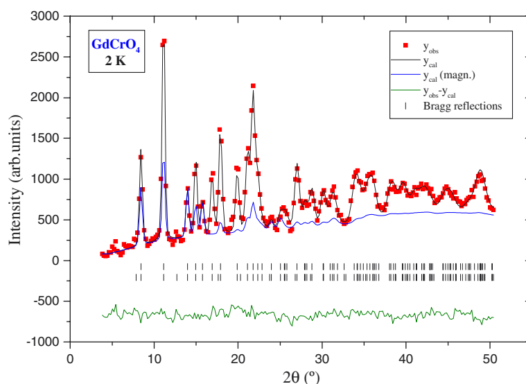
Figure 5. Neutron diffraction pattern of GdCrO 4 at 2 K, refined on the basis of the zircon-type structure and the proposed magnetic structure (see text). The term y_{\text{cal}}(\text{magn.}) denotes the magnetic contribution to the neutron diffraction pattern of GdCrO 4 .
