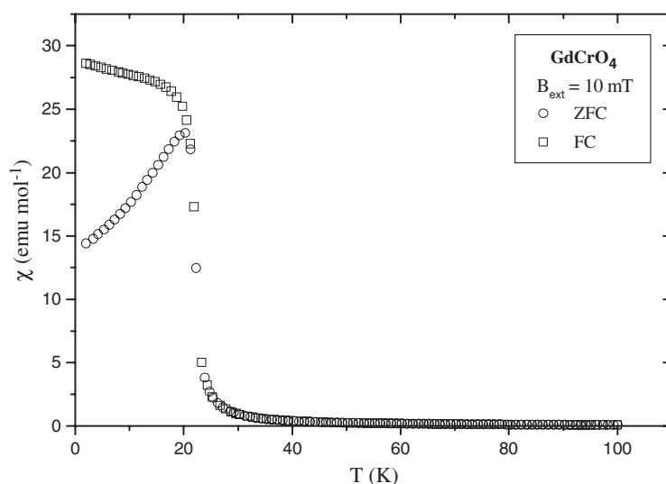
Figure 2. Temperature dependence of the magnetic susceptibility of GdCrO 4 between 2 and 100 K in the presence of an applied magnetic field of \mu_0 H_{\text{ex}} = 10 mT, during the processes of field-cooling (FC) and field-warming after zero-field cooling (ZFC).
