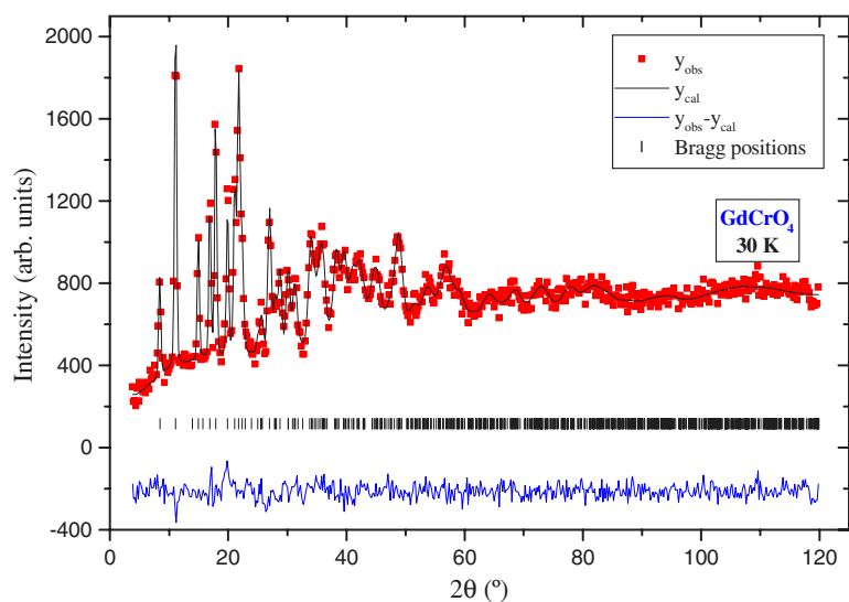
Figure 1. Neutron diffraction pattern of GdCrO 4 at 30 K, refined on the basis of the zircon-type structure.
