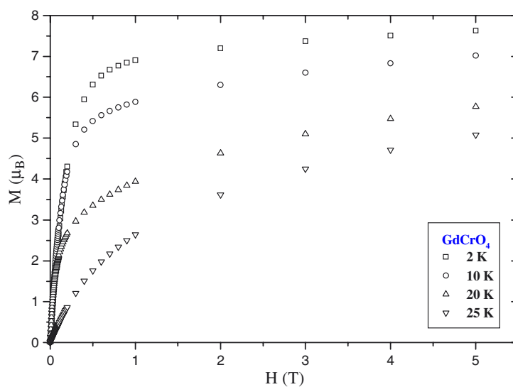
Figure 3. Field-dependent magnetization curves of GdCrO 4 at different measurement temperatures.
